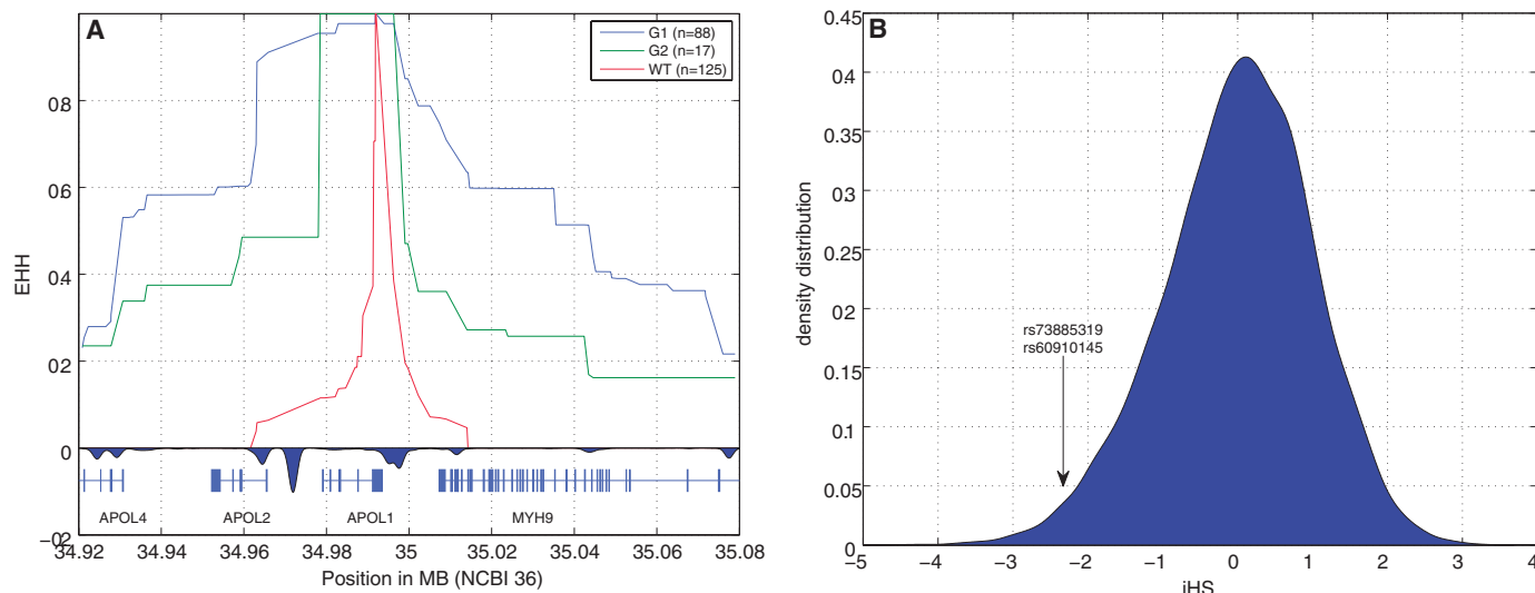
Fig. 2. Natural selection analysis for the Yoruba population. (A) Extended haplotype homozygosity (EHH) values for the three APOL1 alleles [G1, G2, and wild type (WT)]. We computed EHH after combining HapMap3 genotype data with our genotype data for alleles G1 and G2 (table S3), shown together with recombination hotspots around APOL1 . Although APOL1 and MYH9 are in close physical proximity (20 kb apart), they are separated by a recombination hotspot, giving a genetic distance (0.2 cM) equivalent to a physical distance of about 200 kb. (B) Distribution of iHS values in Yoruba, highlighting the iHS value for the SNPs defining G1 (iHS = -2.45). The iHS scores are distributed as a standard normal random variable. Therefore values for which |iHS| > 2 are considered suggestive of selection. (C) Distribution of \Delta iHH values highlighting the SNPs defining allele G1 and allele G2 (for G1, \Delta iHH = 0.471 cM, and for G2, \Delta iHH = 0.275 cM). Values are measured in centimorgans (cM). Raw data are available in table S4.
